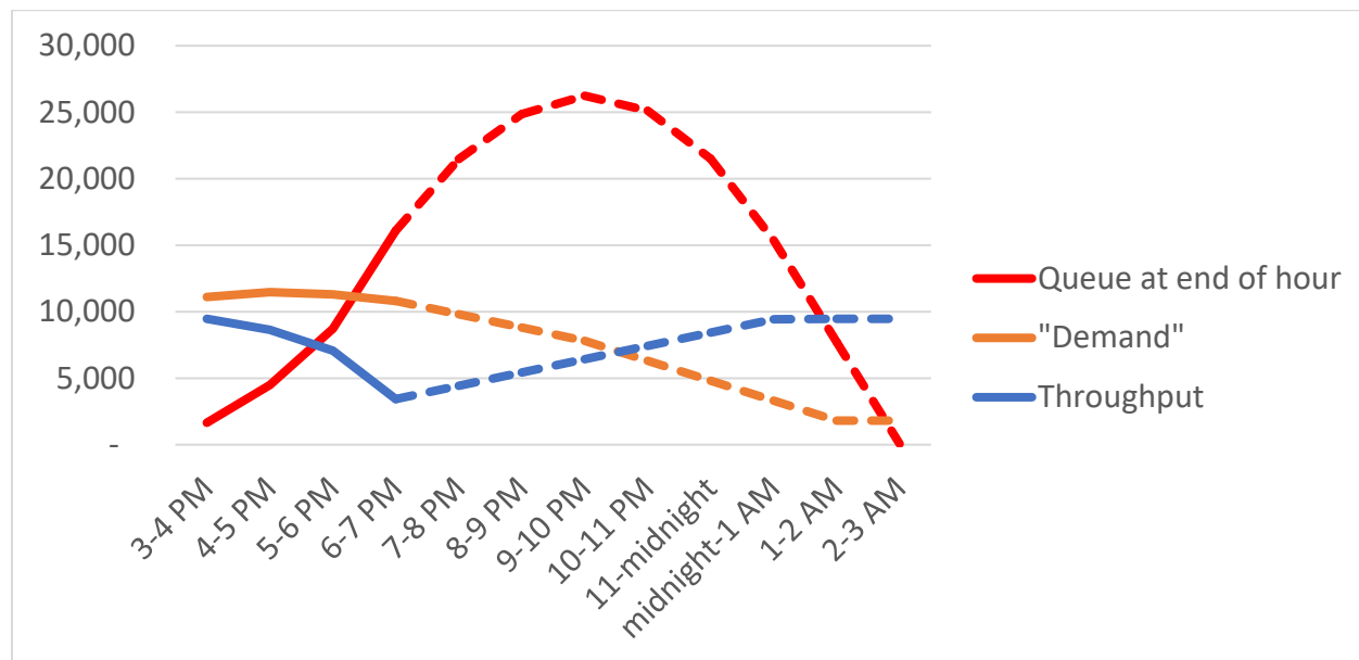
Figure 4: Preferred Alternative 2045 Inner Loop American Legion Bridge Demand, Throughput and Cumulative Unserved Demand (Queue) in the Afternoon Peak Period Illustrative Extension of VISSIM Simulation
